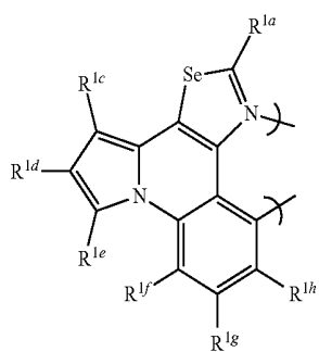
gs9-4
