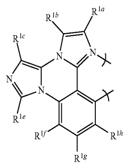
gs3-7
