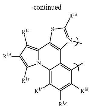
gs9-2
