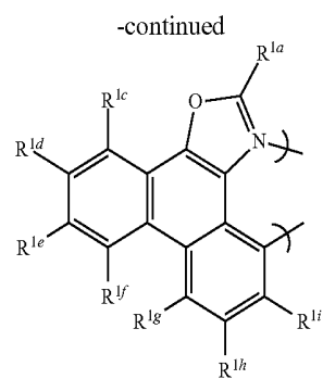
gs9-5
