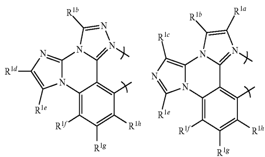
gs3-6
